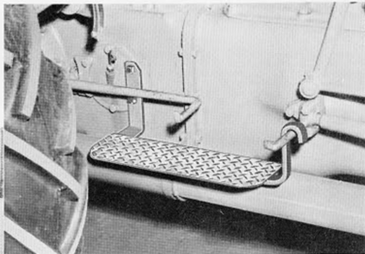
RIGHT STEP INSTALLED ON FORD-FERGUSON TRACTOR
